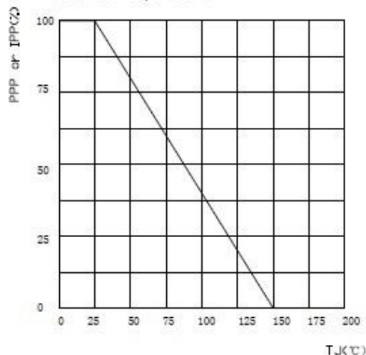
图4: 功率降额曲线 FIG4: Power Derating Curve
