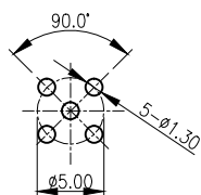
PCB LAYOUT FOR G3401-02000201-00
