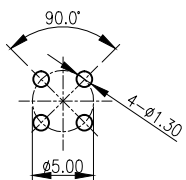
PCB LAYOUT FOR G3401-02000101-00
