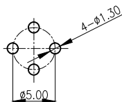
PCB LAYOUT FOR G3401-02000111-00
