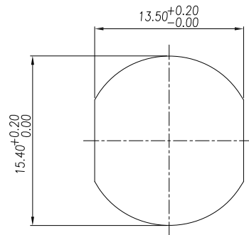
RECOMMENDPANEL CUT-OUT
