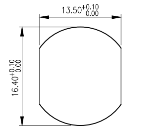
PANEL CUT FOR PANEL THICKNESS MAX OF 4.5mm
