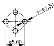
PCB LAYOUT FOR G3402-14000111-00
