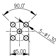
PCB LAYOUT FOR G3402-14000201-00
