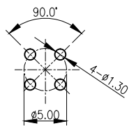
PCB LAYOUT FOR G3402-14000101-00
