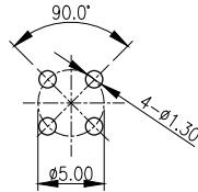
PCB LAYOUT FOR G3401-XXXX0001-00
