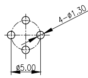
PCB LAYOUT FOR G3401-XXXX0101-00
