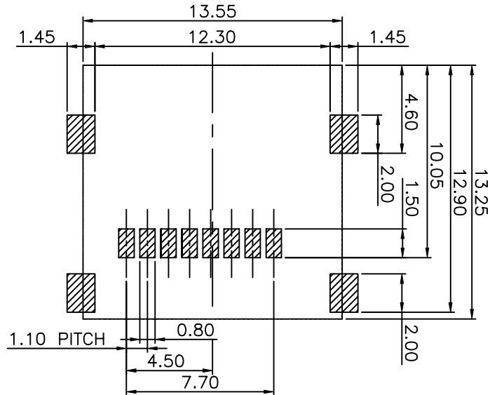
RECOMMENDED PCB LAYOUT (TOP VIEW) TOLERANCE: ±0.05mm
